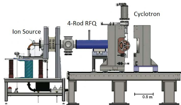
Figure 1: Schematic of the RFQ Test Bench with 1 MeV cyclotron
